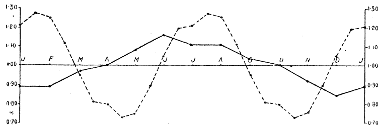
Slight earthquakes.
